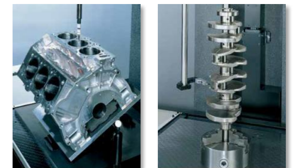
Measurement example of cylinder block and crankshaft.
