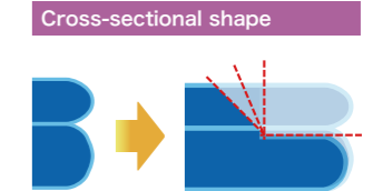
Edge Trimming Bonded Wafer with Special Profile
